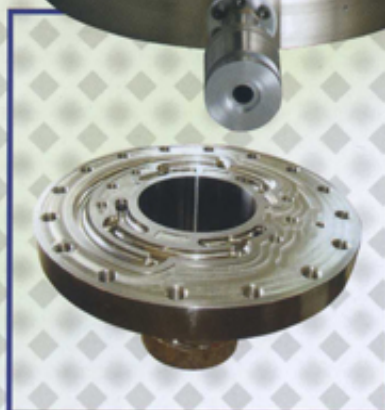
MANUAL SCREEN CHANGER
